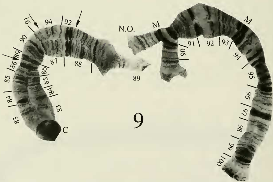
Figs. 8-9. Silk-gland chromosomes of S. parnassum , with landmarks of Rothfels et al. (1978). C = centromere region. 8, Chromosome arm III. Section numbers refer to Simulium parnassum standard banding sequence. Bracket indicates simple inversion relative to Simulium subgeneric standard of Rothfels et al. (1978). Female from Tennessee, Monroe Co., 6 June 1998 (sections 55 through 70) plus female from North Carolina, Haywood Co., 7 June 1998 (section 71). DNA = DNA puff, gB = gray band, Po = polar, St = saw tooth, Sy =
